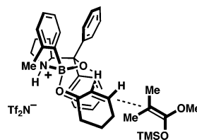
Figure 1. Pre-transition-state assembly for the reaction of 2 , 4 , and S-5 leading to S-6 .
